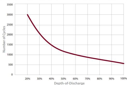
TYPICAL CYCLE LIFE IN A STATIONARY APPLICATION
